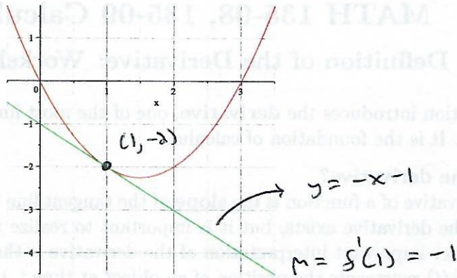
Figure 1: The graph of the function f(x) = x^2 - 3x along with the tangent line at the point x = 1 .
