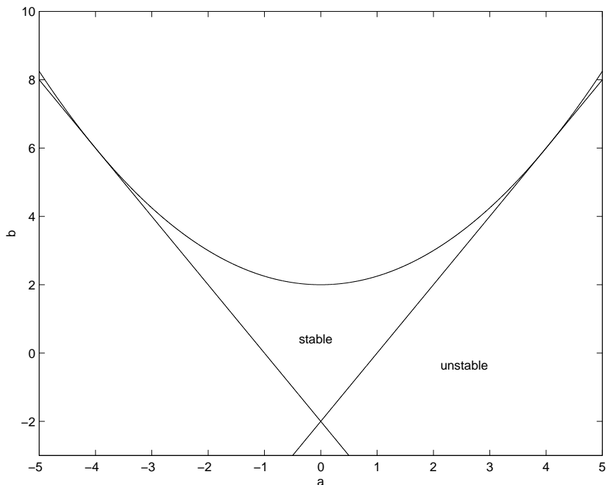
Figure 1: Stability region for \lambda^4 + a\lambda^3 + b\lambda^2 + a\lambda + 1 in the ab -plane. The period doubling boundary is b = 2a - 2 and the Krein collision curve is the parabola b = a^2/4 + 2 .
