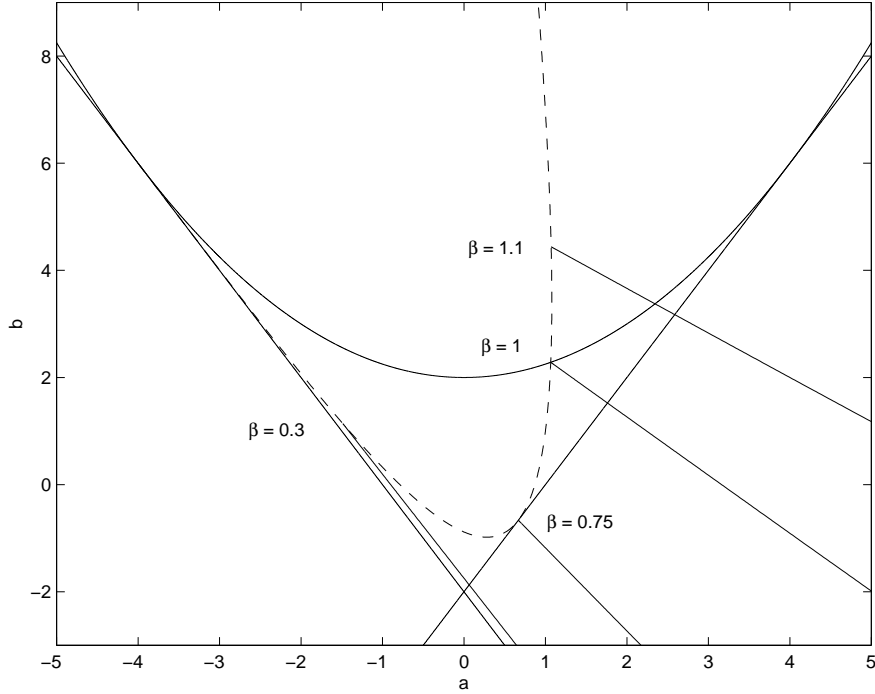
Figure 4: Examining the multiplier curves for fixed \beta and increasing eccentricity e in the ab -plane. Remarkably, the curves are almost linear.
