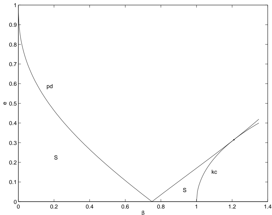
Figure 3: The linear stability diagram in terms of the parameters \beta and e . There are two regions of linear stability labeled S. The period doubling curve (pd) reaches the \beta -axis at \beta = 3/4 . The Krein collision curve (kc) begins at \beta = 1 and is tangent to the period doubling curve at the point (1.209133, 0.314508) , where all four multipliers are -1 .
