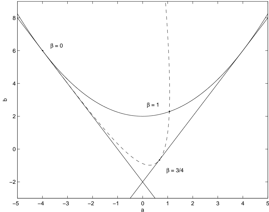
Figure 2: Stability diagram for the case e = 0 . The dashed curve describes the characteristic multipliers. Two key \beta -values are \beta = 3/4 , where two multipliers are -1 and \beta = 1 , where the two pairs of multipliers meet on the unit circle. Stability is lost for \beta > 1 .
